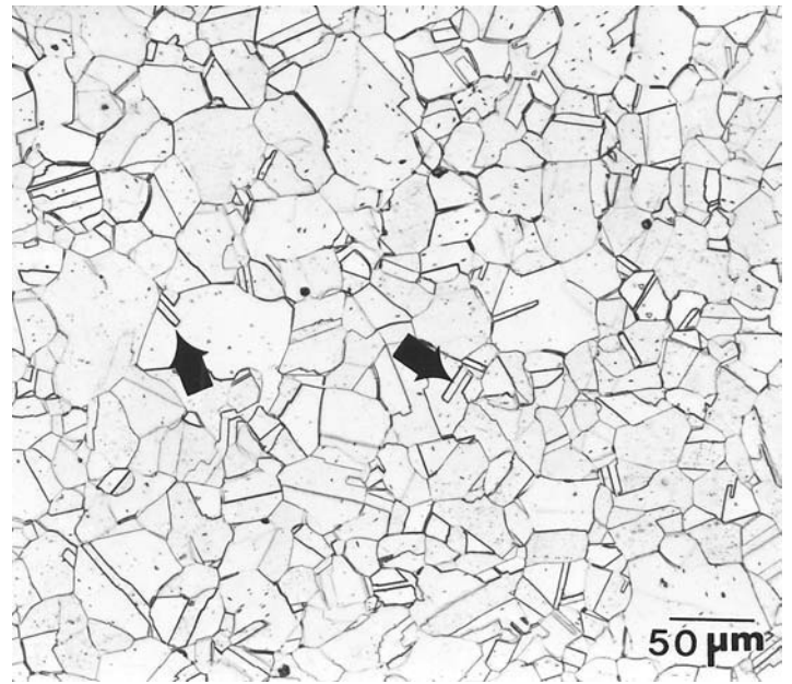
Fig. 1.22 Micrograph of a low-expansion steel (Invar) showing a microstructure consisting of austenite. The straight-edged regions (arrows) are annealing twins. Etched in 4% picral. 200×
