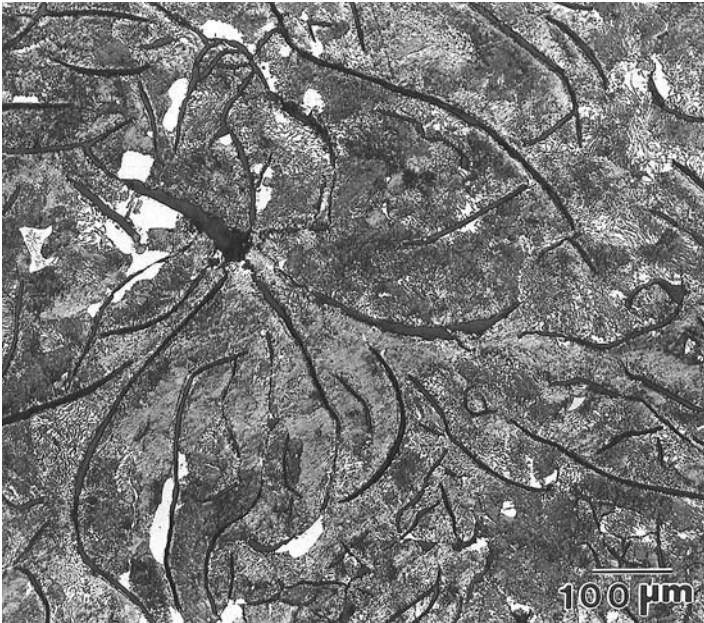
Fig. 1.24 Micrograph of a gray cast iron showing a microstructure consisting of pearlite (gray etching constituent), ferrite (light etching constituent), and graphite flakes (dark constituent). Etched in 4% picral. 100×
