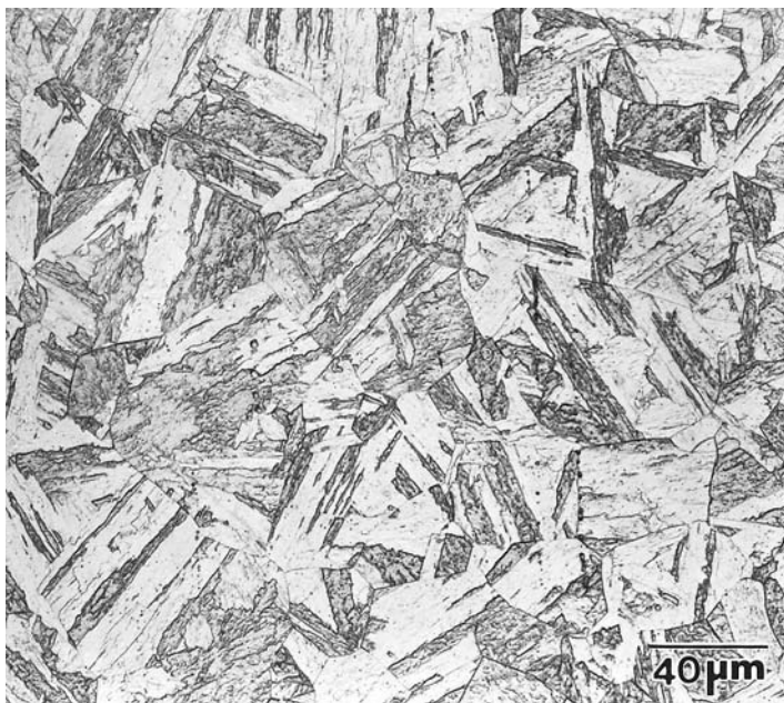
Fig. 1.17 Micrograph of a precipitation-hardening stainless steel (Custom 630) showing a microstructure consisting of martensite. Etched in Fry's reagent. 320×
