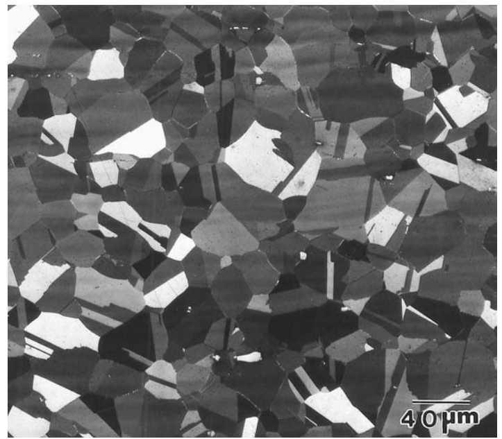
Fig. 1.18 Micrograph of an iron-base superalloy A286 showing a microstructure consisting of austenite. The straight-edged regions are annealing twins. Etched in a solution of 100 ml water, 20 ml HCl, 1 g \text{NH}_4\text{F} HF, and 0.5 g \text{K}_2\text{S}_2\text{O}_5 . 200×
