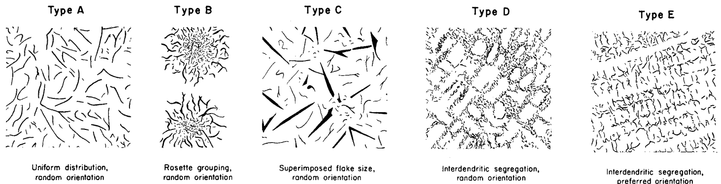
Fig. 1.25 Types of graphite flakes in gray iron (American Foundryman's Society-ASTM). In the recommended practice (ASTM A 247), these charts are shown at a magnification of 100 \times . They have been reduced to one-third size for reproduction here.
