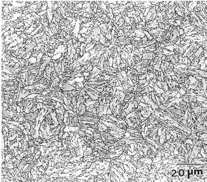
Fig. 1.15 Micrograph of AISI 410 martensitic stainless steel showing a microstructure consisting of 100% martensite. Etched in Kalling's No. 1 reagent. 500×
