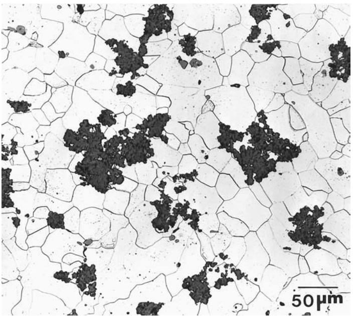
Fig. 1.28 Micrograph of a malleable cast iron showing a microstructure consisting of ferrite (light etching constituent) and temper carbon (dark gray irregular-shaped constituent). Etched in 2% nital. 200×
