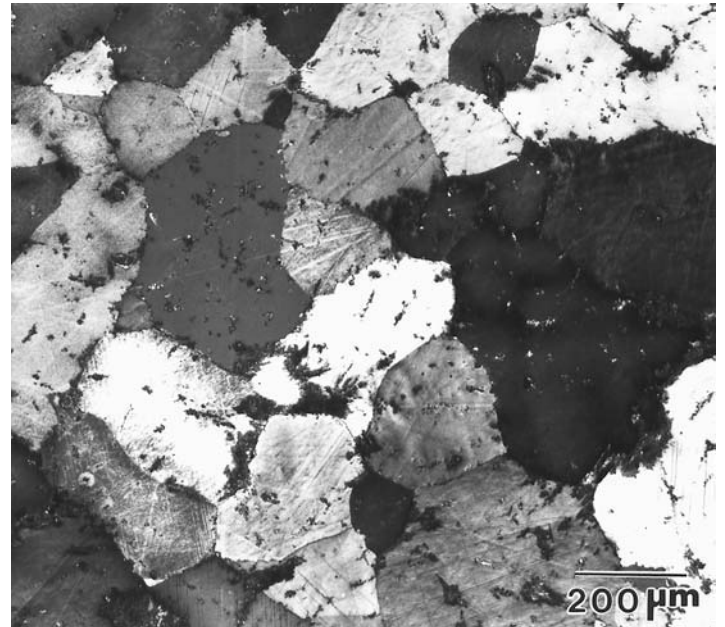
Fig. 1.20 Micrograph of ASTM A 128 austenitic manganese steel (Hadfield steel) casting showing a microstructure consisting of austenite. Etched in 2% nital (5 s) followed by removal of the stain in aqueous 3% EDTA and etching in 20% sodium metabisulfite solution. 64×
