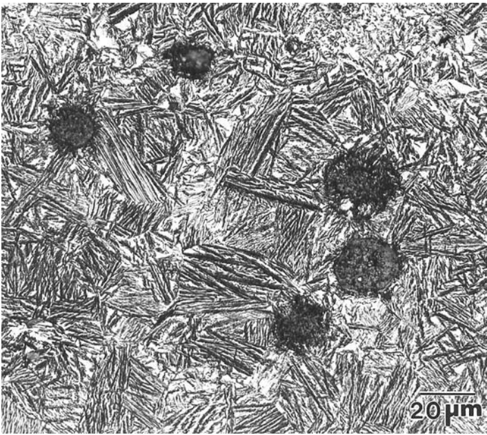
Fig. 1.31 Micrograph of an austempered ductile cast iron showing a microstructure consisting of bainite (acicular constituent) and graphite nodules (dark gray constituent). Etched in 2% nital. 500×
