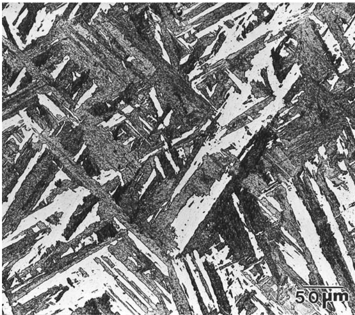
Fig. 1.21 Micrograph of a maraging steel showing a microstructure consisting of martensite. Etched in Kalling No. 1. 200×
