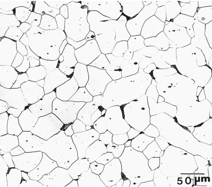
Fig. 1.2(a) Micrograph of low-carbon AISI/SAE 1010 steel showing a matrix of ferrite grains (white etching constituent) and pearlite (dark etching constituent). Etched in Marshall's reagent followed by 2% nital. 200X
