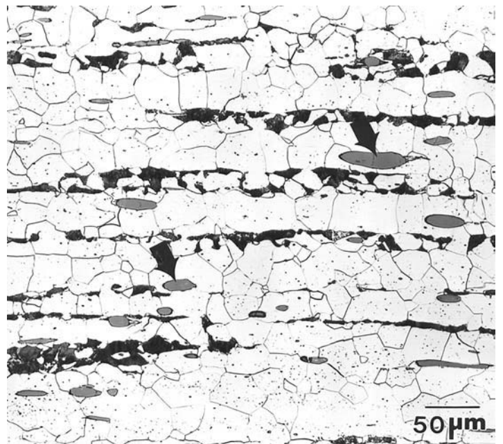
Fig. 1.3 Micrograph of a resulfurized, rephosphorized AISI/SAE 1213 steel showing manganese sulfide inclusions (the gray, oblong particles marked by arrows). The remaining microstructure is ferrite (white etching constituent) and pearlite (dark etching constituent). Etched in 4% picral followed by 2% nital. 200×
