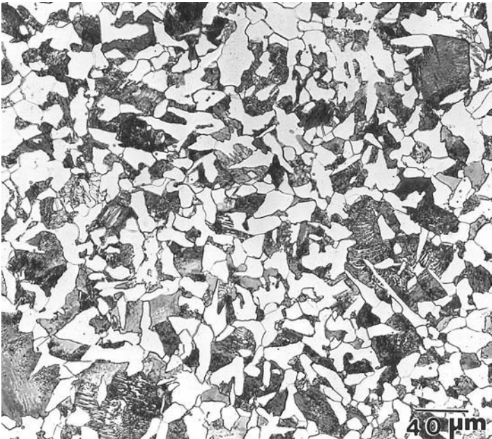
Fig. 1.2(b) Micrograph of medium-carbon AISI/SAE 1040 steel showing ferrite grains (white etching constituent) and pearlite (dark etching constituent). Etched in 4% picral followed by 2% nital. 300X
