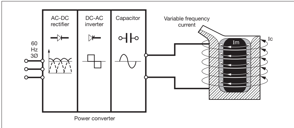
Fig 5 Basic electric circuit for a medium frequency coreless furnace
